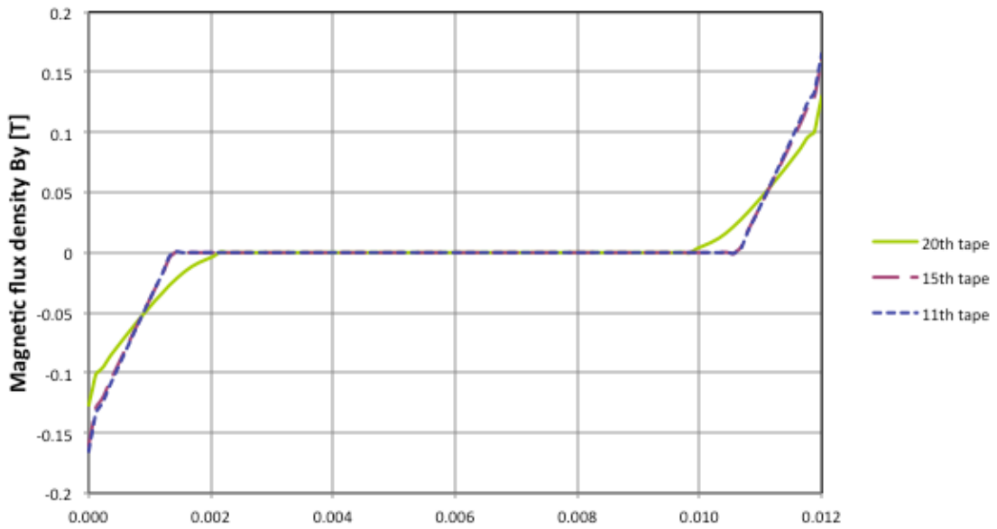
Magnetic flux penetration (150 A, n = 25)
