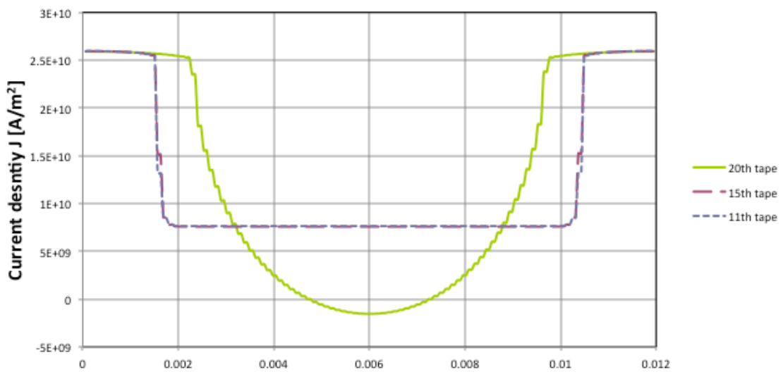
Current distribution (150 A, n =101)
