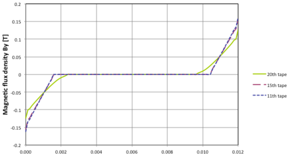
Magnetic flux penetration (150 A, n = 101)
