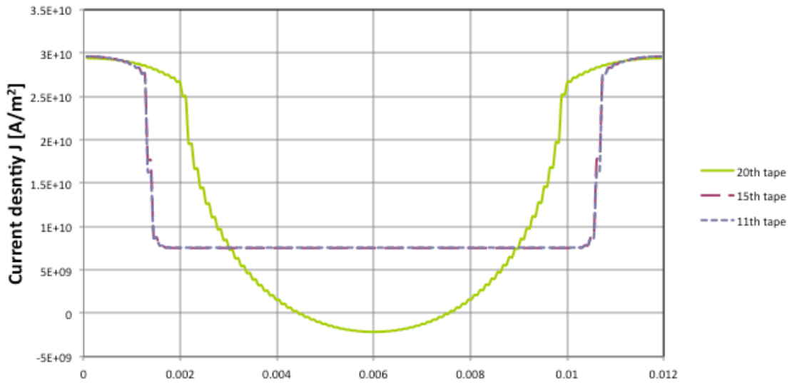
Current distribution (150 A, n =25)
